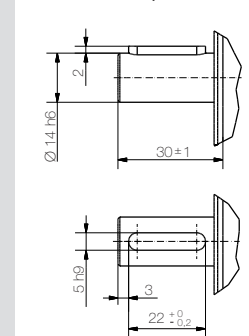
Passfeder (optional)
