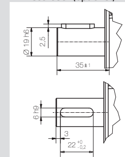
Passfeder (optional)
